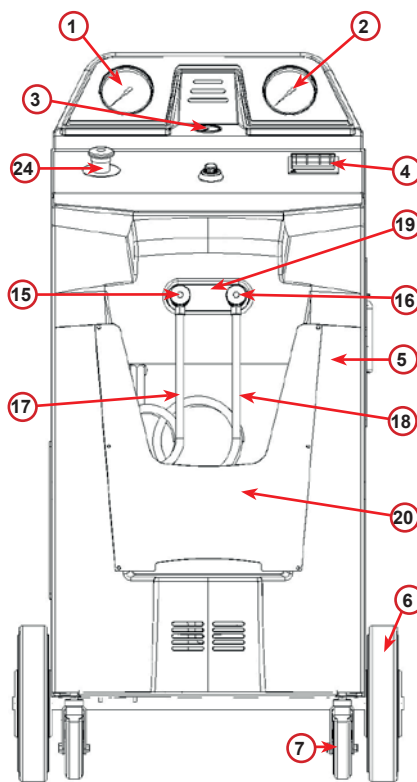
fig. 002 Front view
