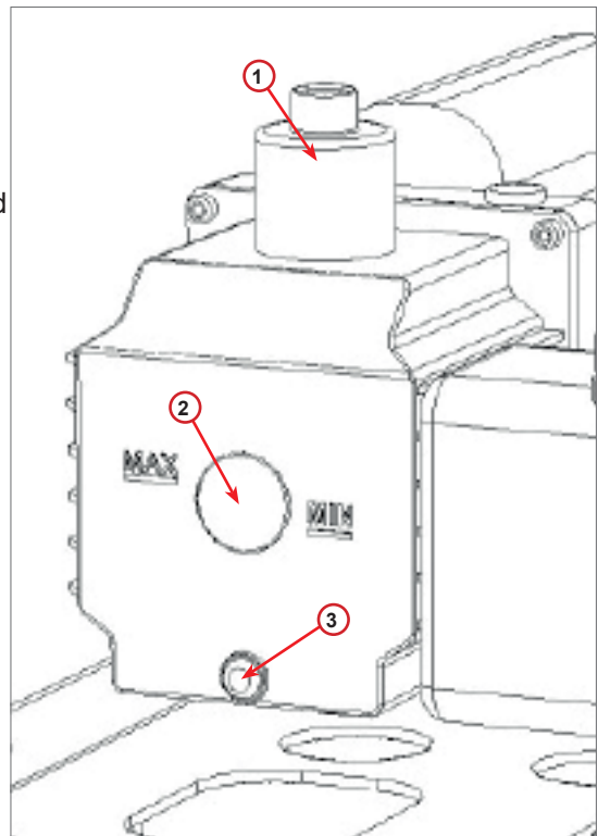
fig. 008 Vacuum pump
